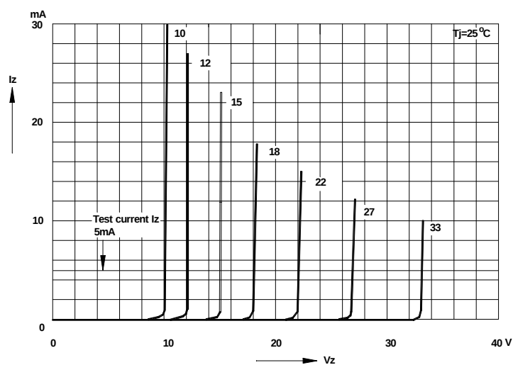
Breakdown characteristics
